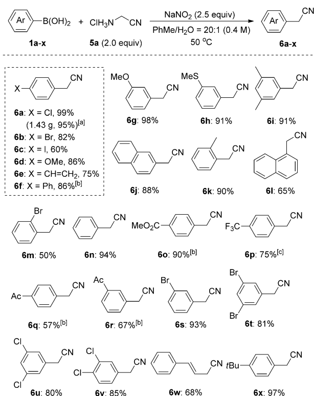
Scheme 5. Reaction of arylboronic acids with \alpha -aminoacetonitrile hydrochloride ( 5a ). If not otherwise noted, the reaction was carried out with 1 (0.5 mmol) and 5a (1.0 mmol) in \text{PhMe}/\text{H}_2\text{O} (20:1; 1.25 mL) at 50^\circ\text{C} . All the yields refer to those of the isolated products. [a] Reaction was scaled up to 10 mmol of 1a and 20 mmol of 5a . [b] The reaction was carried out at 100^\circ\text{C} with DCE as solvent instead of \text{PhMe} . [c] The reaction was carried out at 100^\circ\text{C} .
