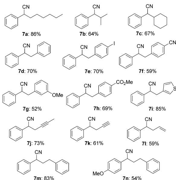
Scheme 6. Reaction of phenylboronic acids and aminoacetone nitrile derivatives. The reaction was carried out with 1n or 1d (0.5 mmol) and 5b–n (1.0 mmol) in PhMe/H 2 O (20:1; 1.25 mL) at 25 °C. All the yields refer to those of the isolated products.
